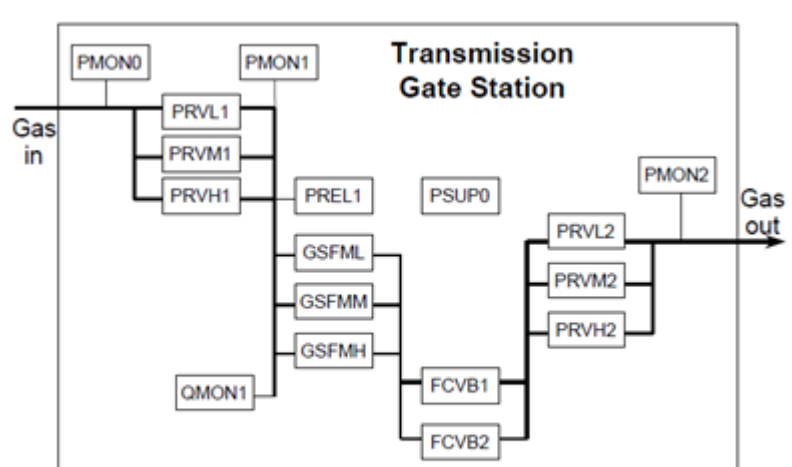
Figure 3-3 The Logical Device for a Transmission Gate Station May Have Many Bricks
